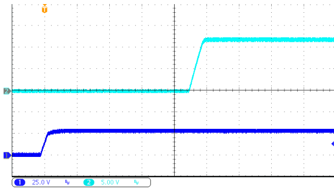
Main output voltage (blue) (5 V/div) Input voltage (navy blue) (25 V/div) Time base: 20 ms/div
