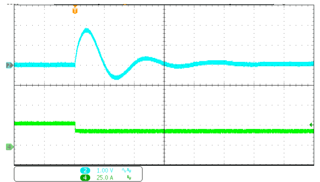
Main output voltage (blue) (1 V/div) Output current (green) (25 A/div) Time base: 4 ms/div
