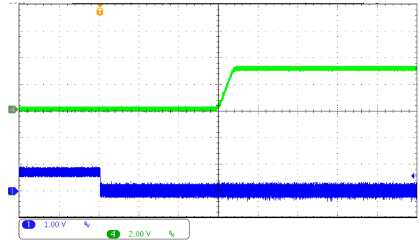
Aux output voltage (green) (2 V/div) ENABLE* (navy blue) (1V/div) Time base: 10 ms /div
