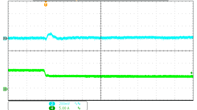
Aux output voltage (blue) (200 mV/div) Time base: 40 μs/div Output current (green) (5 A/div)
