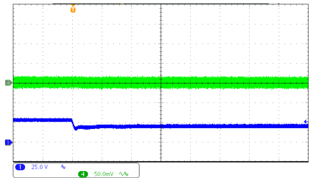
Aux output voltage (green) (50 mV/div) Time base: 4 ms/div Input voltage (navy blue) (25 V/div)
