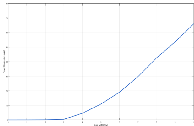
Figure Q. Non-operating power dissipation versus input voltage, ENABLE* and INHIBIT* de-asserted
