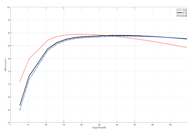
Figure T. Efficiency versus output power at minimum, nominal and maximum input voltage
