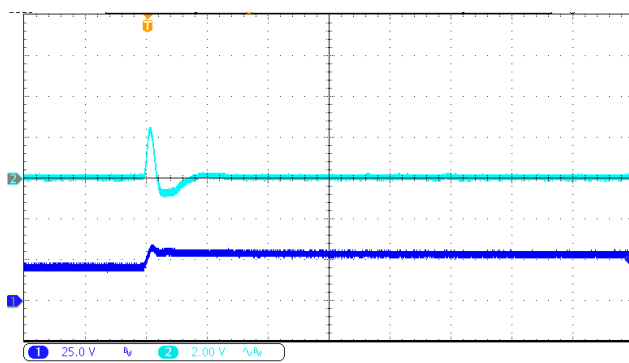
Main output voltage (blue) (2 V/div) Input voltage (navy blue) (25 V/div) Time base: 4 ms/div
