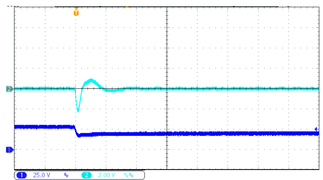
Main output voltage (blue) (2 V/div) Input voltage (navy blue) (25 V/div) Time base: 4 ms/div
