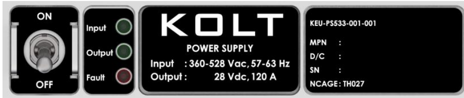
Figure 26. English Label Option Front View
