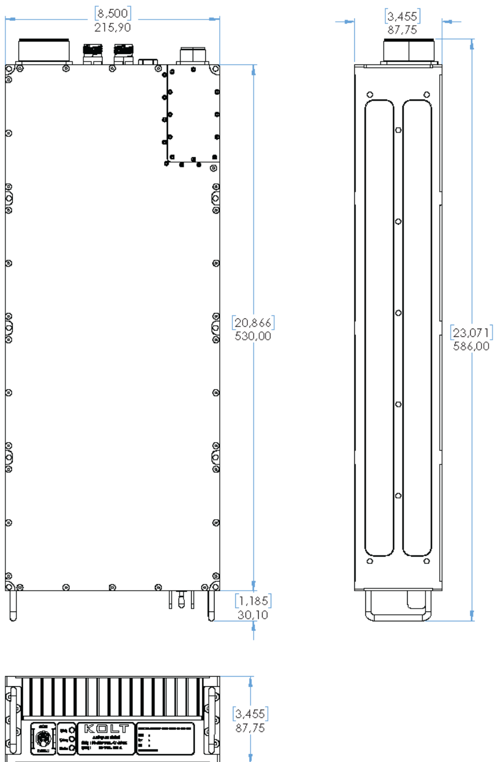
Figure 28. Mechanical Dimensions
