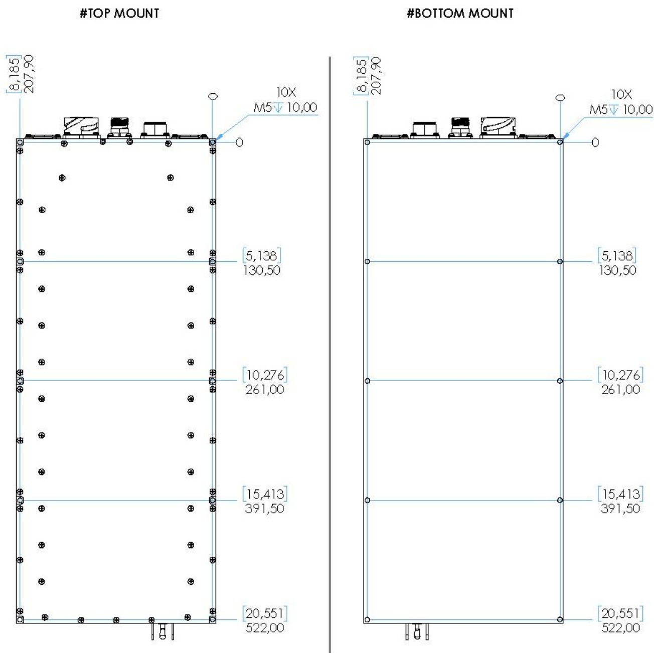
Figure 27. Mounting Details and Mounting Holes Coordinates
