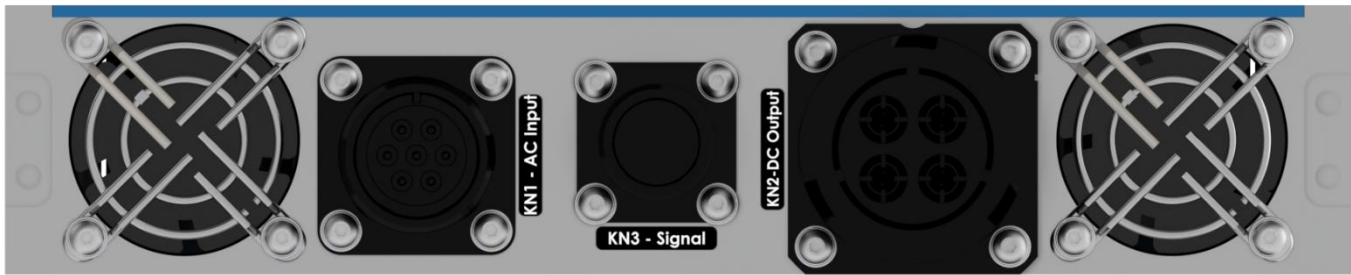
Figure 17. Connector Panel
