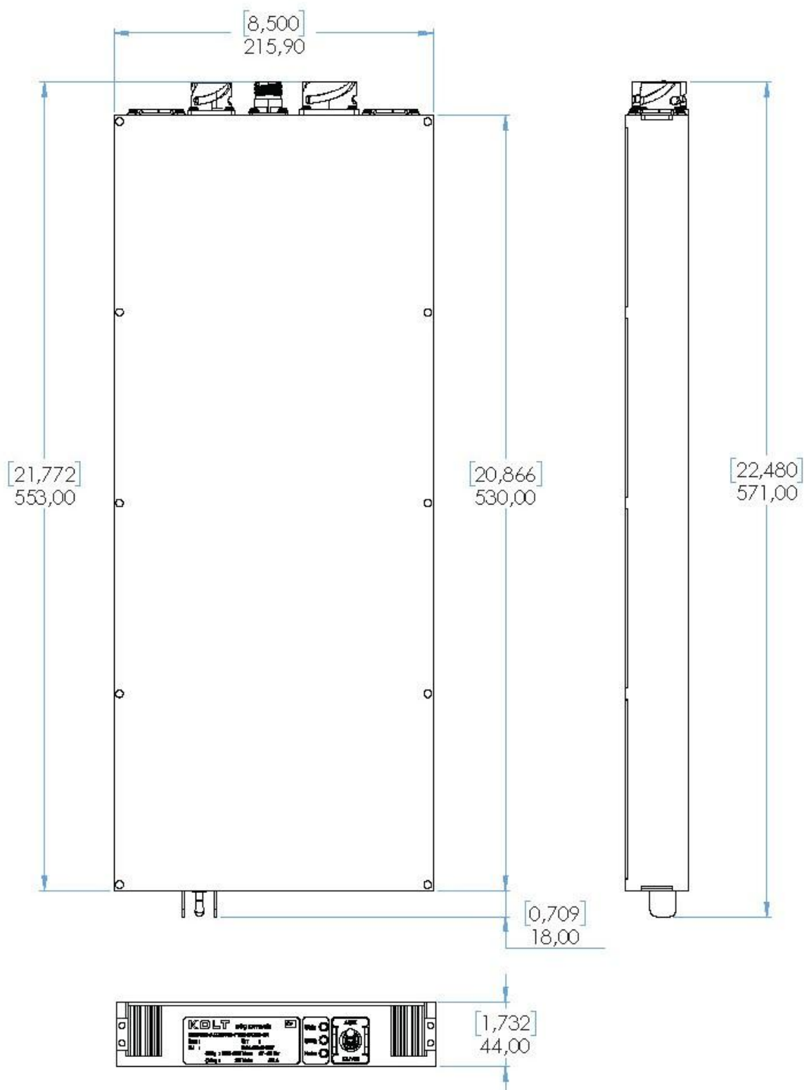
Figure 26. Mechanical Dimensions
