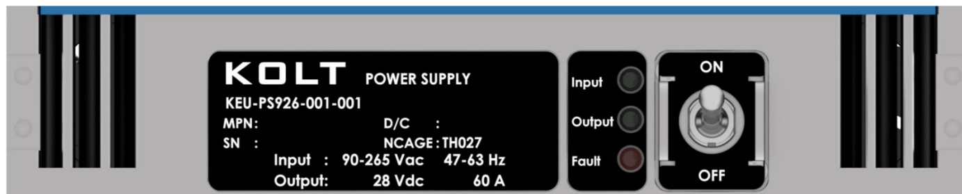
Figure 21. Front Panel
