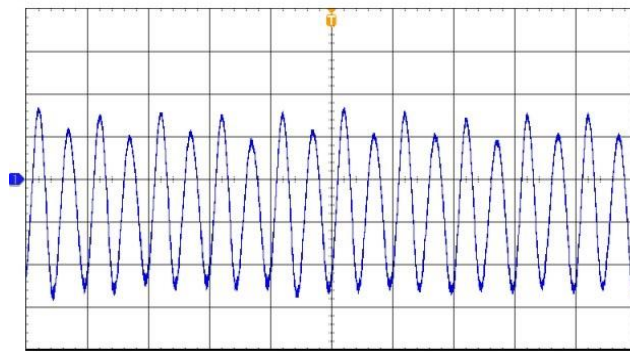
Output voltage (navy blue) (50 mV/div) Time base: 10 μs/div
