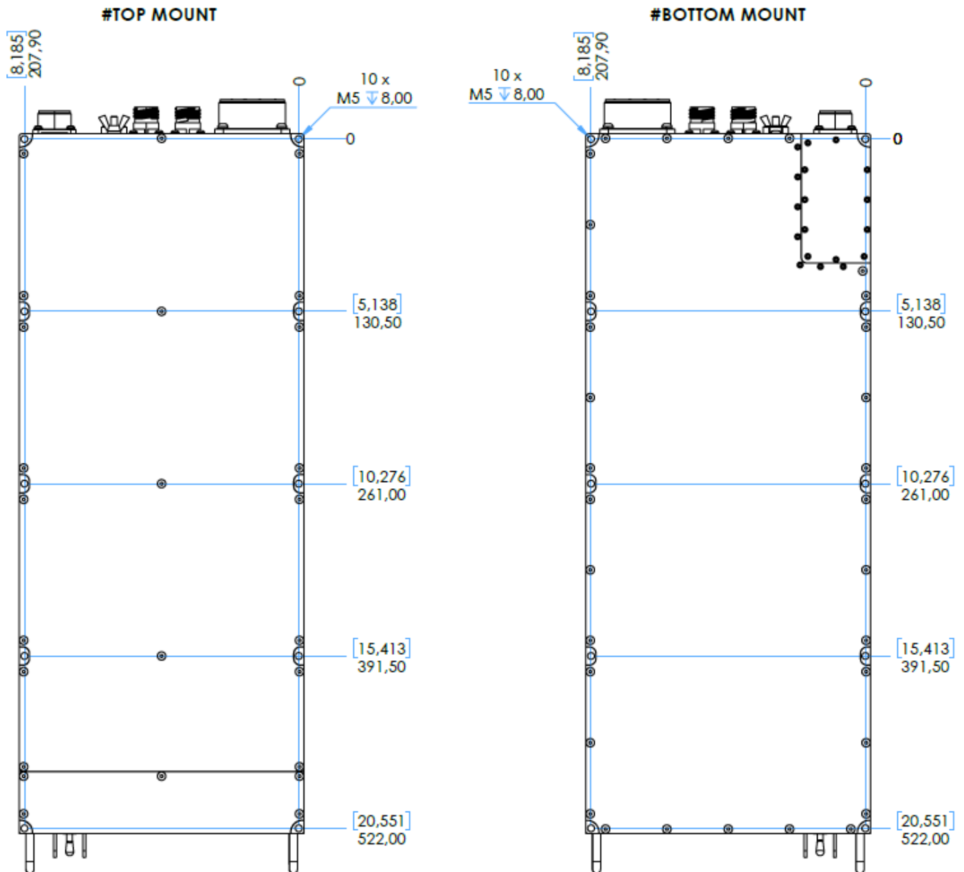
Figure 28. Mounting Details and Mounting Holes Coordinates
