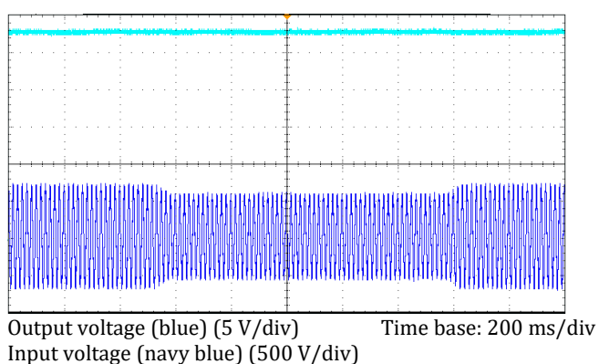
Figure 9. Line transient response: from 485 V_{LL\_RMS} to 395 V_{LL\_RMS} and back to 485 V_{LL\_RMS} at nominal output voltage (DC Coupled)
