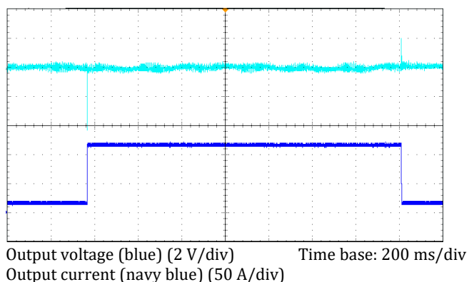
Figure 8. Zoomed in view of load transient response: from 10% to 100% and back to 10% at nominal output voltage (AC Coupled)
