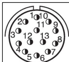
Figure 20. Signal Connector View
