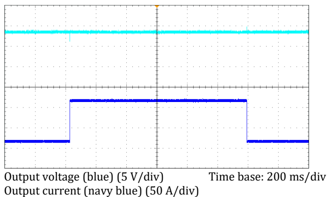
Figure 7. Load transient response: from 10% to 100% and back to 10% at nominal output voltage (DC Coupled)
