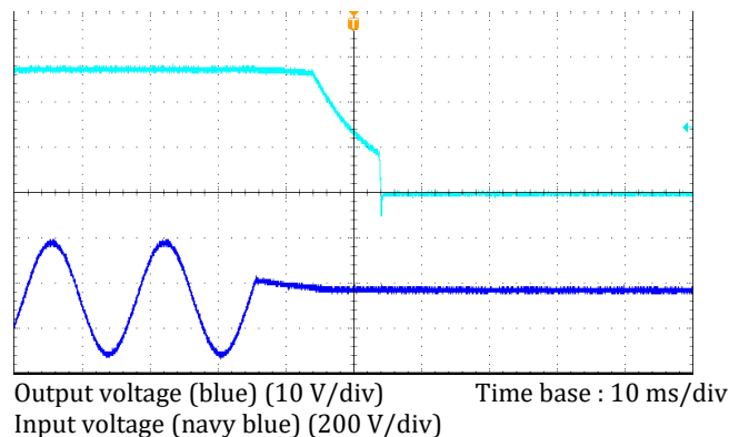
Figure 12. Hold-up waveform at rated load current and nominal output voltage
