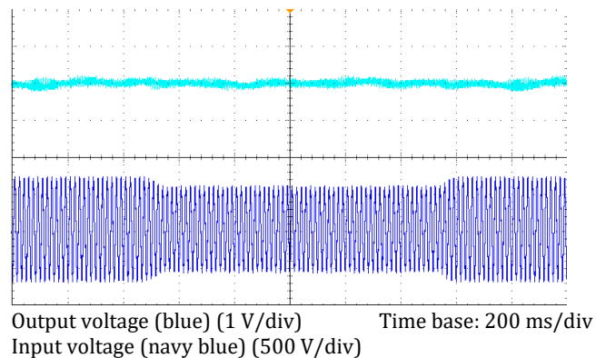
Figure 10. Zoomed in view of line transient response: from 485 V_{LL\_RMS} to 395 V_{LL\_RMS} and back to 485 V_{LL\_RMS} at nominal output voltage (AC Coupled)
