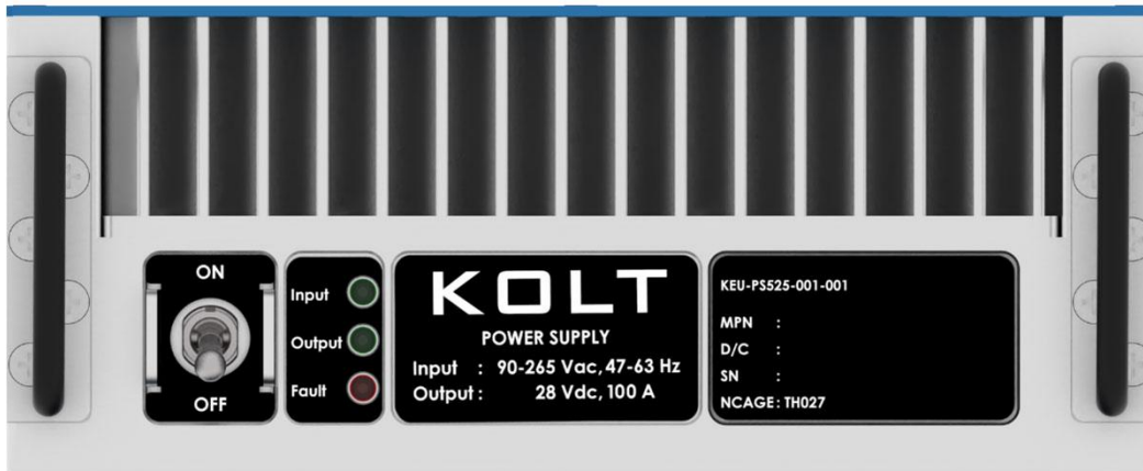
Figure 23. Front Panel
