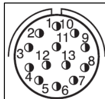
Figure 21. Signal Connector View
