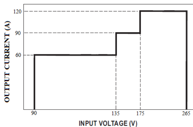
Figure 17. Derating curve of output load versus input voltage
