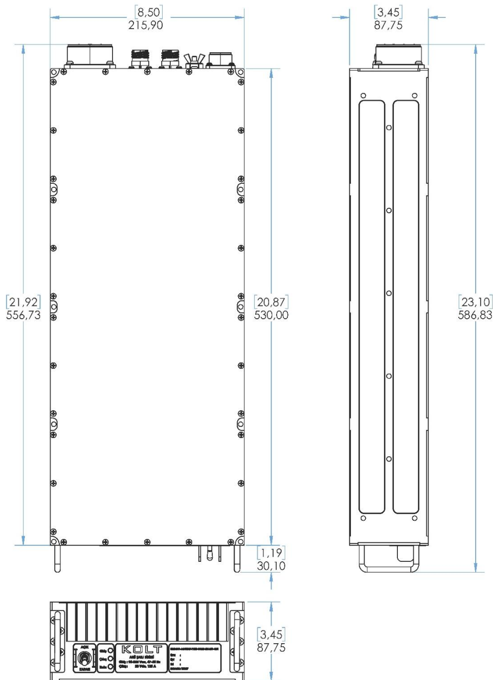
Figure 28. Mechanical Dimensions
