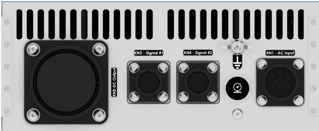
Figure 18. Connector Panel
