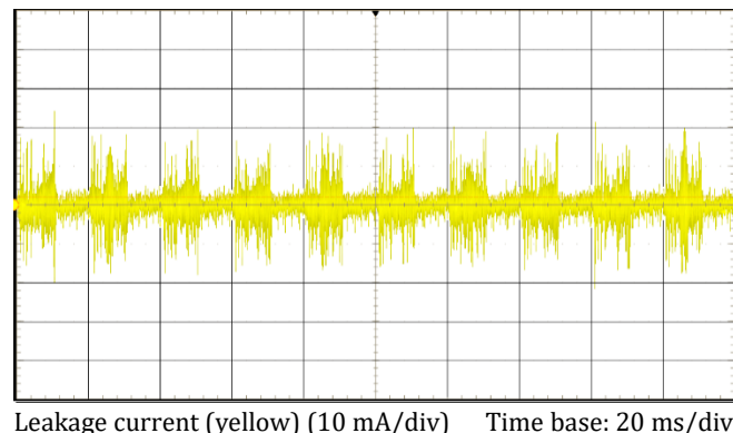
Figure 4. Leakage current to ground at nominal input voltage and 10% load current
