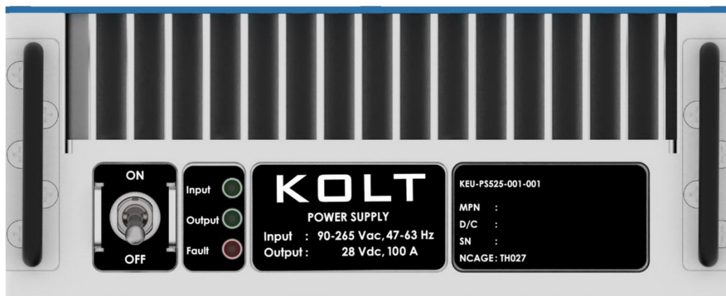
Figure 23. Front Panel
