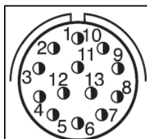
Figure 22. Signal Connector View
