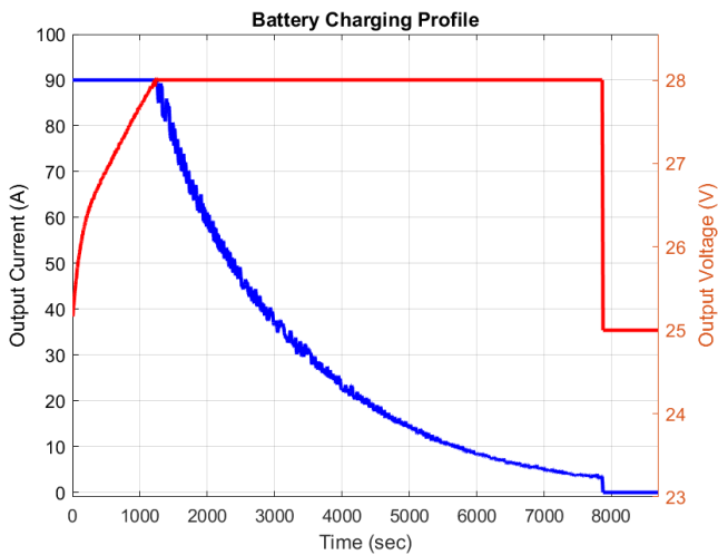
Figure 1. Battery charging profile based on measured battery current and battery voltage data. Power delivered is 2520 W.
