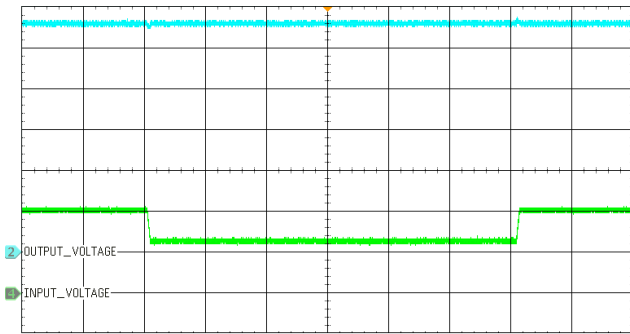
Output voltage (blue) (5 V/div) Time base : 200 ms/div Input voltage (green) (200 V/div)
