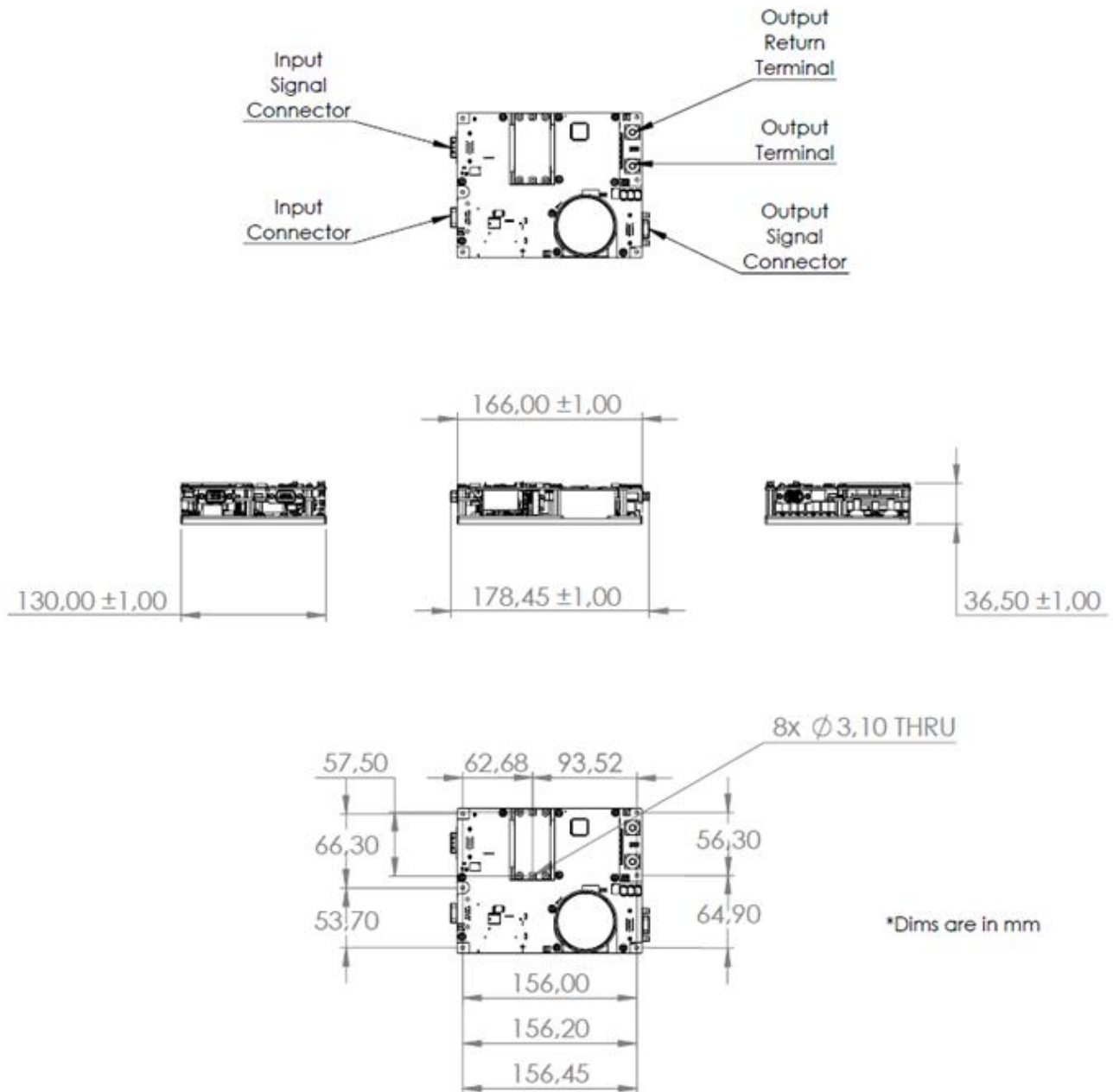
Figure 12. Mechanical Dimensions
