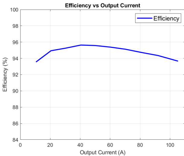
Figure 8. Efficiency versus output current at nominal input voltage
