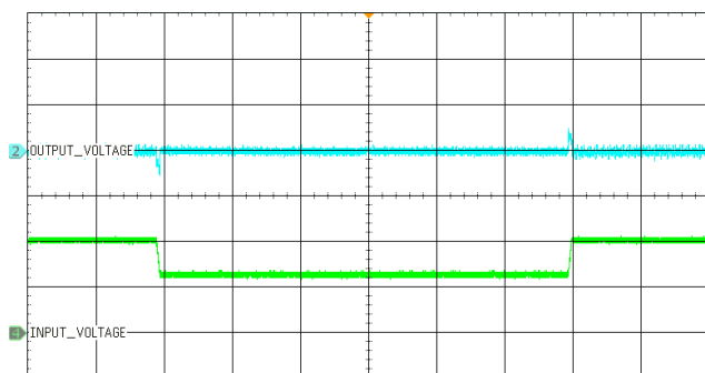
Output voltage (blue) (1 V/div) Time base : 200 ms/div Output current (green) (200 V/div)
