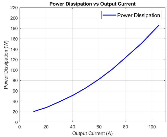
Figure 10. Power dissipation versus output current at nominal input voltage
