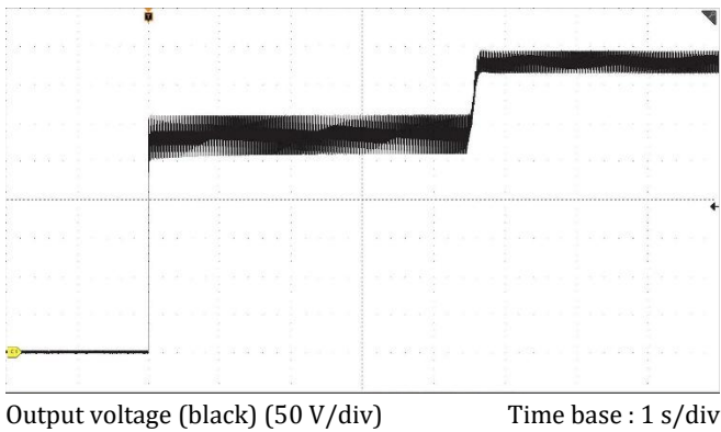
Figure 13. Start-up waveform at rated load current and nominal output voltage
