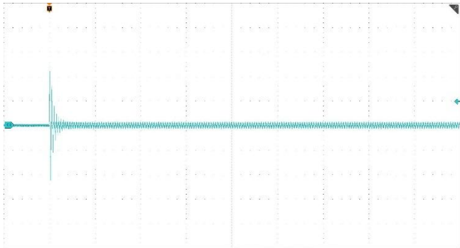
Input current (navy blue) (20 A/div) Time base : 400 ms/div
