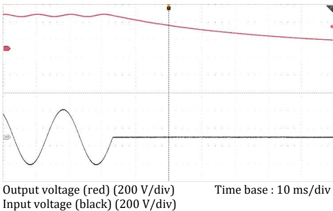
Figure 14. Hold-up waveform at rated load current and nominal output voltage
