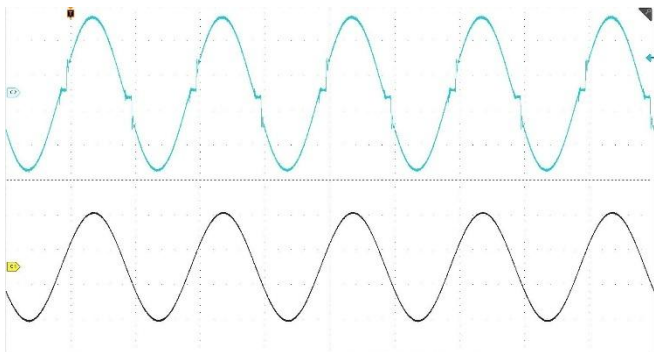
Input voltage (navy blue) (200 V/div) Time base : 10 ms/div Input current (black) (10 A/div)
