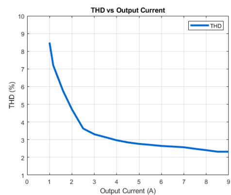
Figure 18. Total harmonic distortion (THD) versus output current at nominal input voltage
