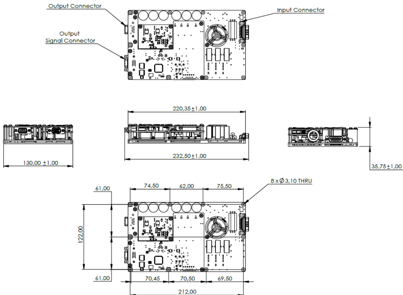
Figure 19. Mechanical Dimensions
