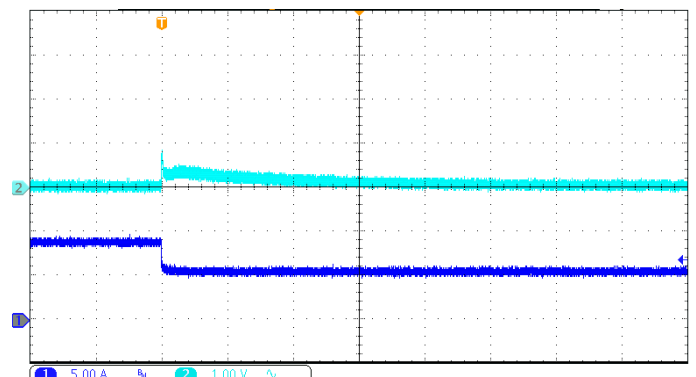
Output voltage (blue) (1 V/div) Time base: 200 \mu\text{s} /div Output current (navy blue) (5 A/div)
