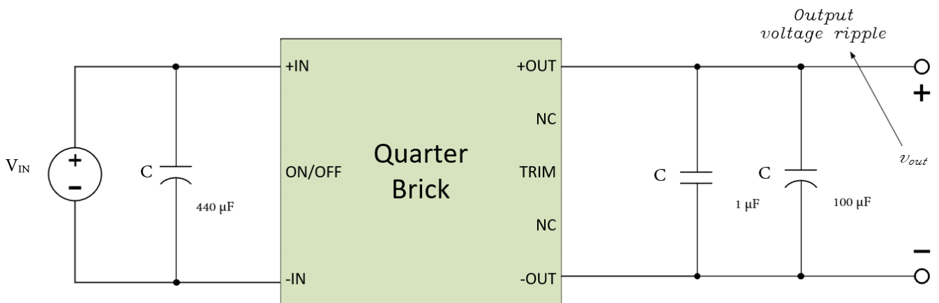
Figure 12. Test set-up showing measurement point for output voltage ripple.
