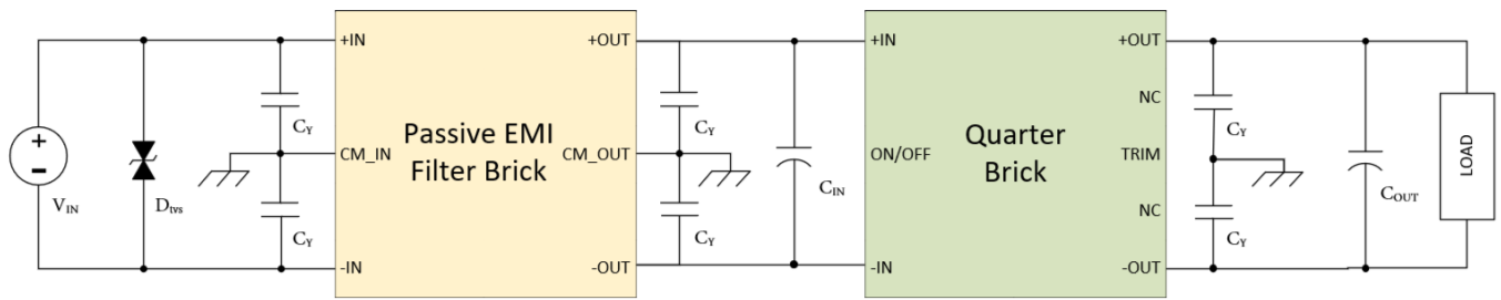
Figure 20. Recommended Application for better EMI/EMC compliance
