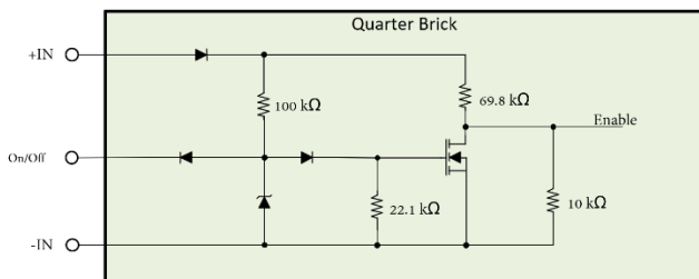
Figure 13. Internal ON/OFF Circuit
