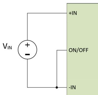
Figure 14. Recommended ON State Connection
