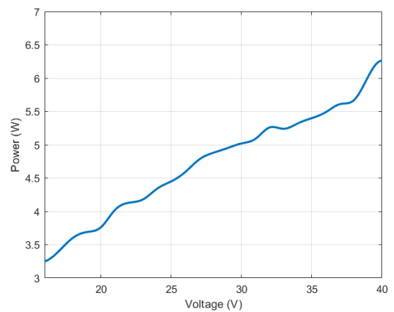
Figure 10. Enabled power dissipation versus input voltage
