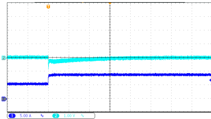
Output voltage (blue) (1 V/div) Time base: 200 \mu\text{s} /div Output current (navy blue) (5 A/div)
