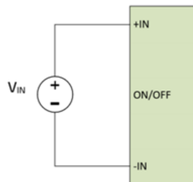
Figure 15. Recommended OFF State Connections
