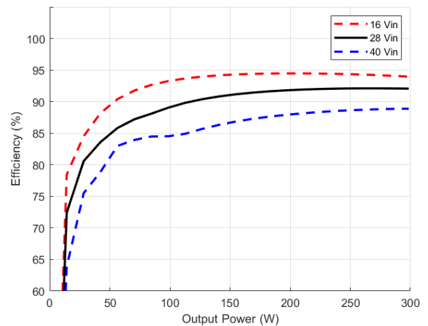
Figure 11. Efficiency versus output power at minimum, nominal, and maximum input voltage
