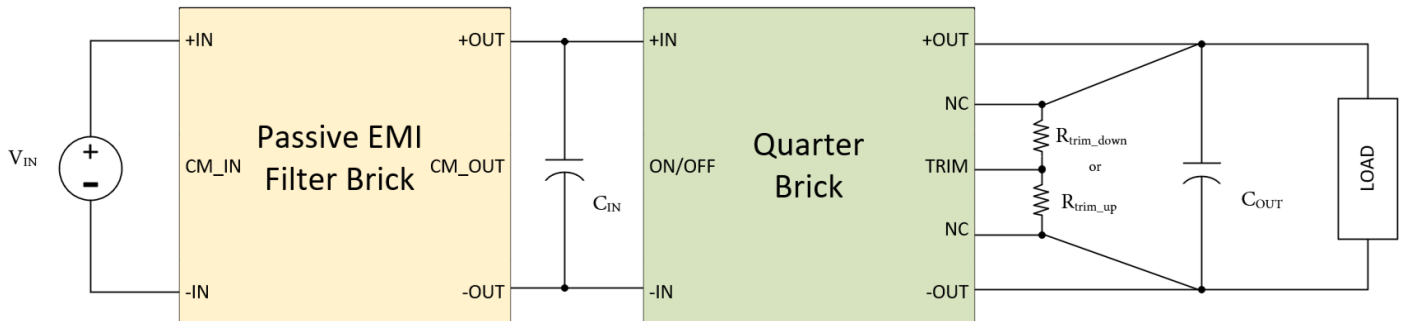
Figure 18. Typical Application
