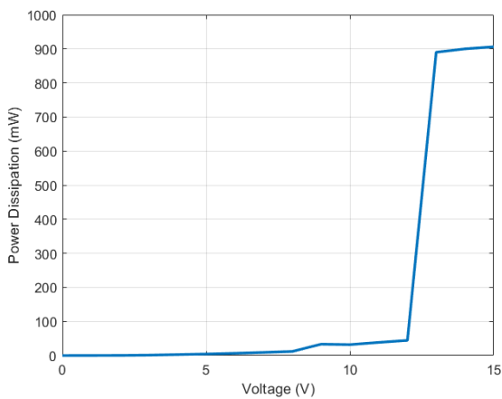
Figure 7. Disabled power dissipation versus input voltage
