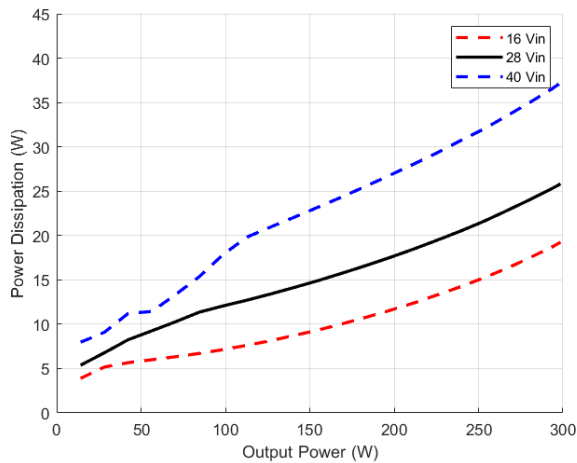
Figure 8. Power dissipation versus output power at minimum, nominal, and maximum input voltage
