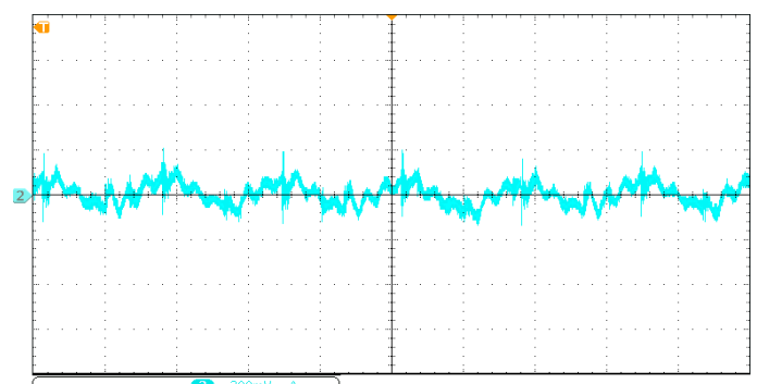
Output voltage ripple (200 mV/div) Time base: 2 \mu\text{s} /div
