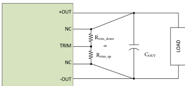
Figure 16. Typical Trim Application Circuit
