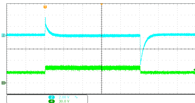
Output voltage (blue) (2 V/div) Time base: 10 ms/div Input voltage (green) (30 V/div)
