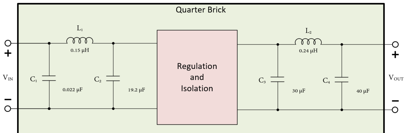
Figure 21. Internal input and output filter diagram of Quarter Brick
