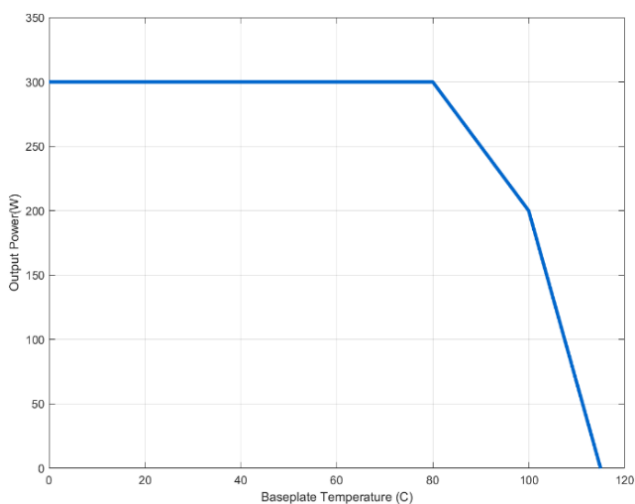
Figure 9. Thermal Derating (maximum output power vs baseplate temperature) at nominal input voltage
