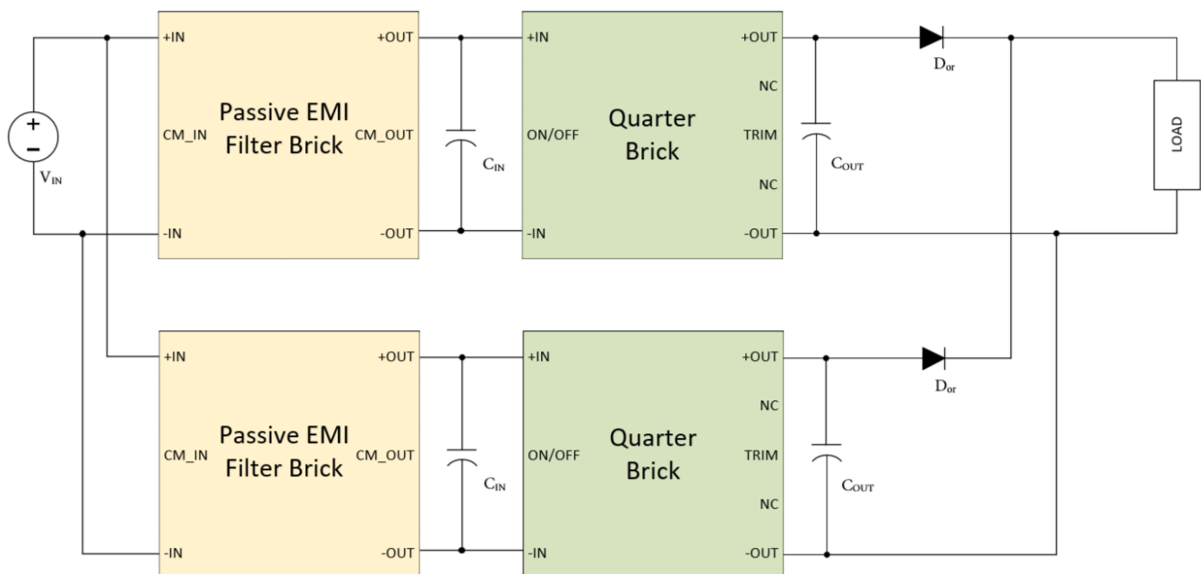
Figure 19. Recommended Application N+1 Redundant Parallel Connection
