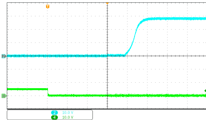
Output voltage (blue) (10 V/div) Time base: 10 ms/div ON/OFF pin voltage (green) (10 V/div)
