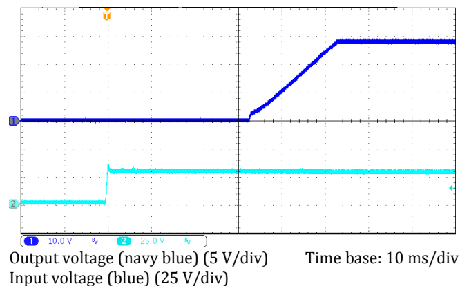
Figure D. Turn on transient at full resistive load with 1 \mu F ceramic and 100 \mu F electrolytic capacitor across the load terminals.
