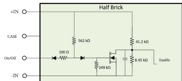
Figure Q. Internal ON/OFF circuit of Negative Logic Option
