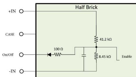
Figure N. Internal ON/OFF circuit of Positive Logic Option
