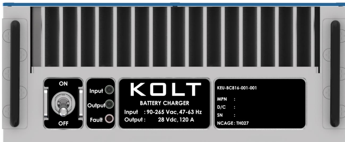
Figure 23. Front Panel
