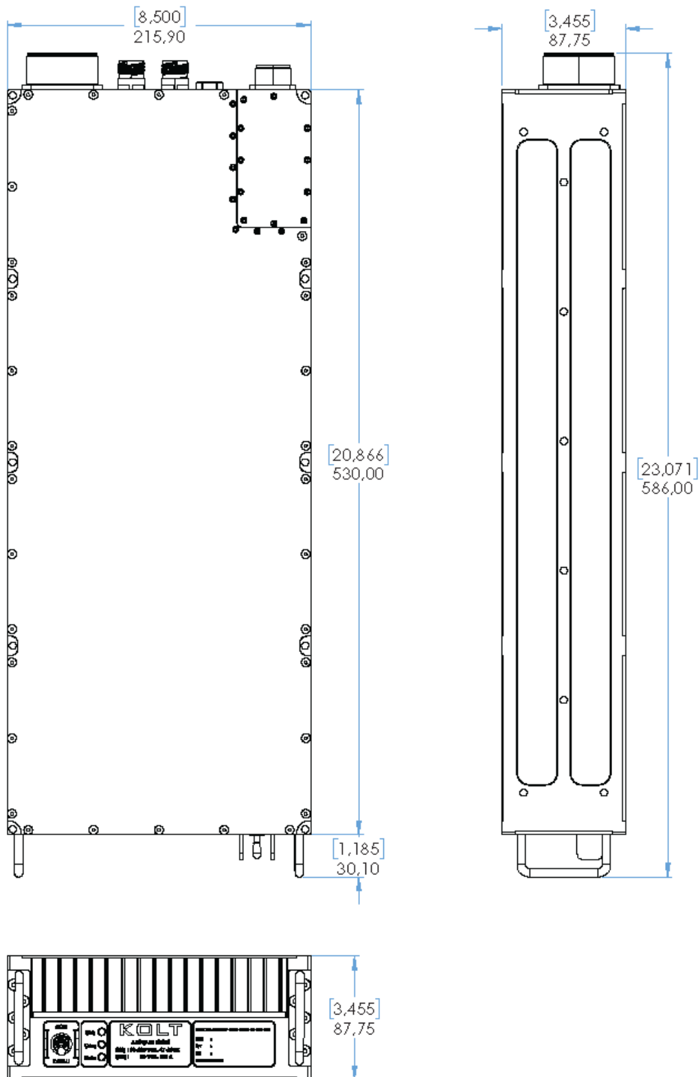
Figure 28. Mechanical Dimensions
