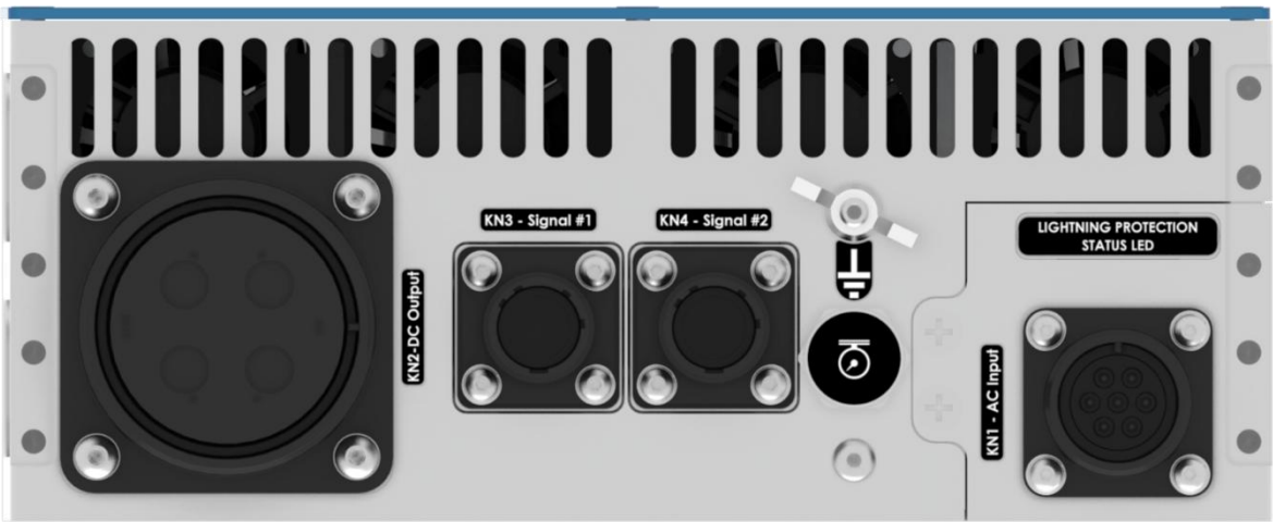
Figure 18. Connector Panel
