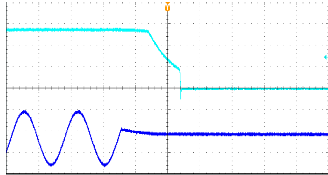
Output voltage (blue) (10 V/div) Time base: 10 ms/div Input voltage (navy blue) (200 V/div)
