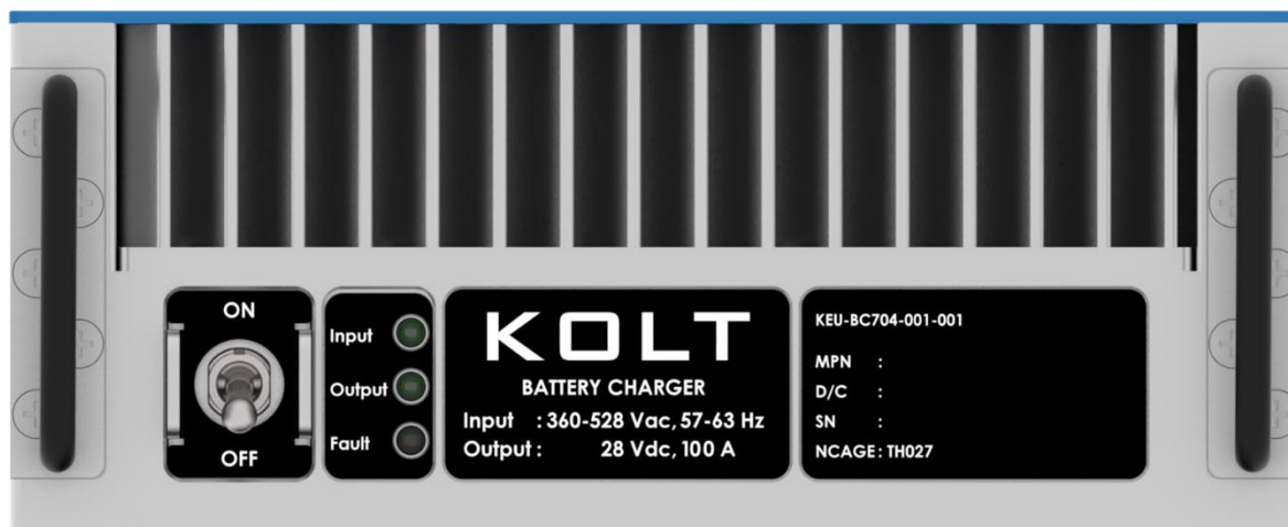
Figure 22. Front Panel
