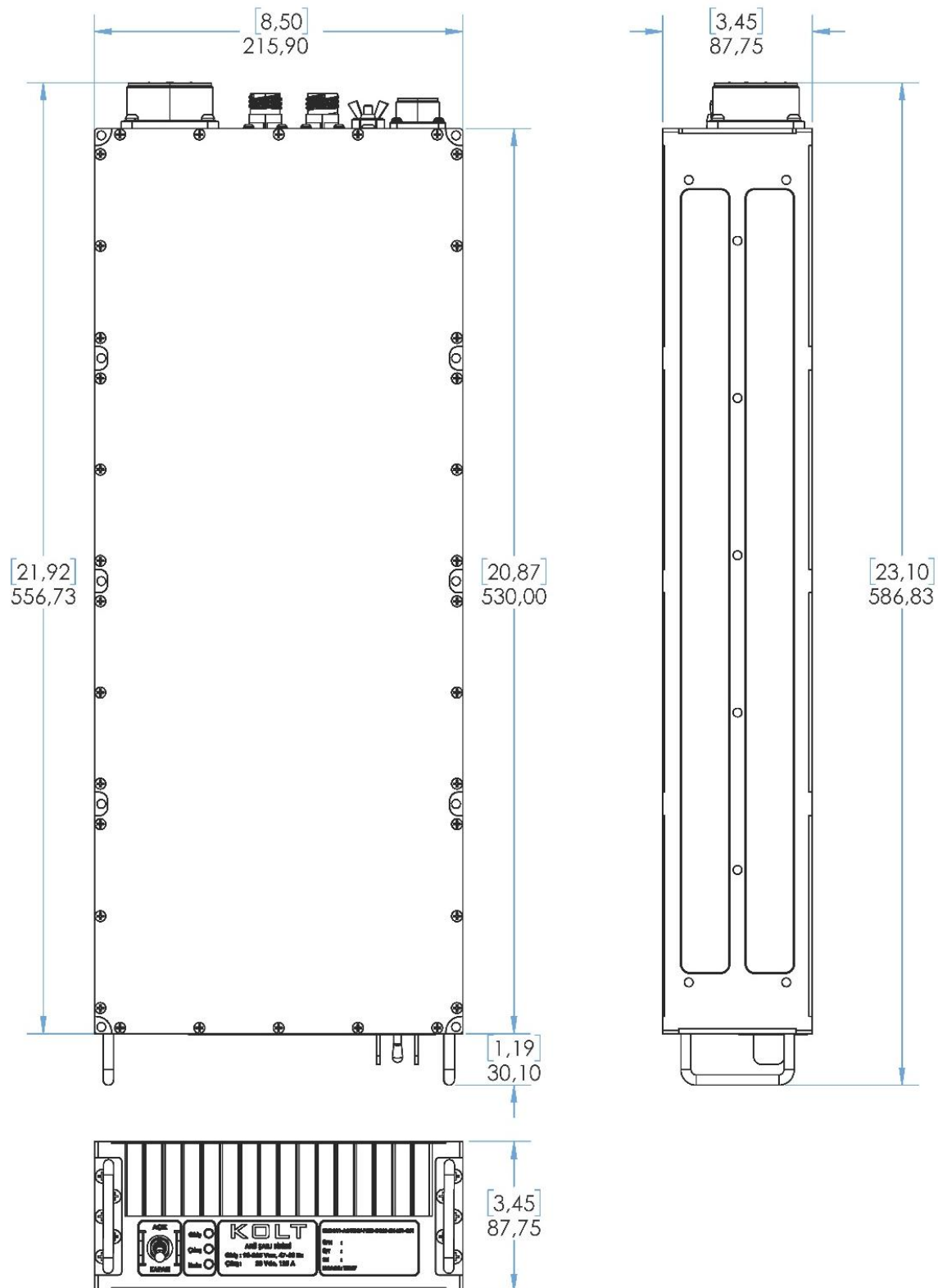
Figure 27. Mechanical Dimensions
