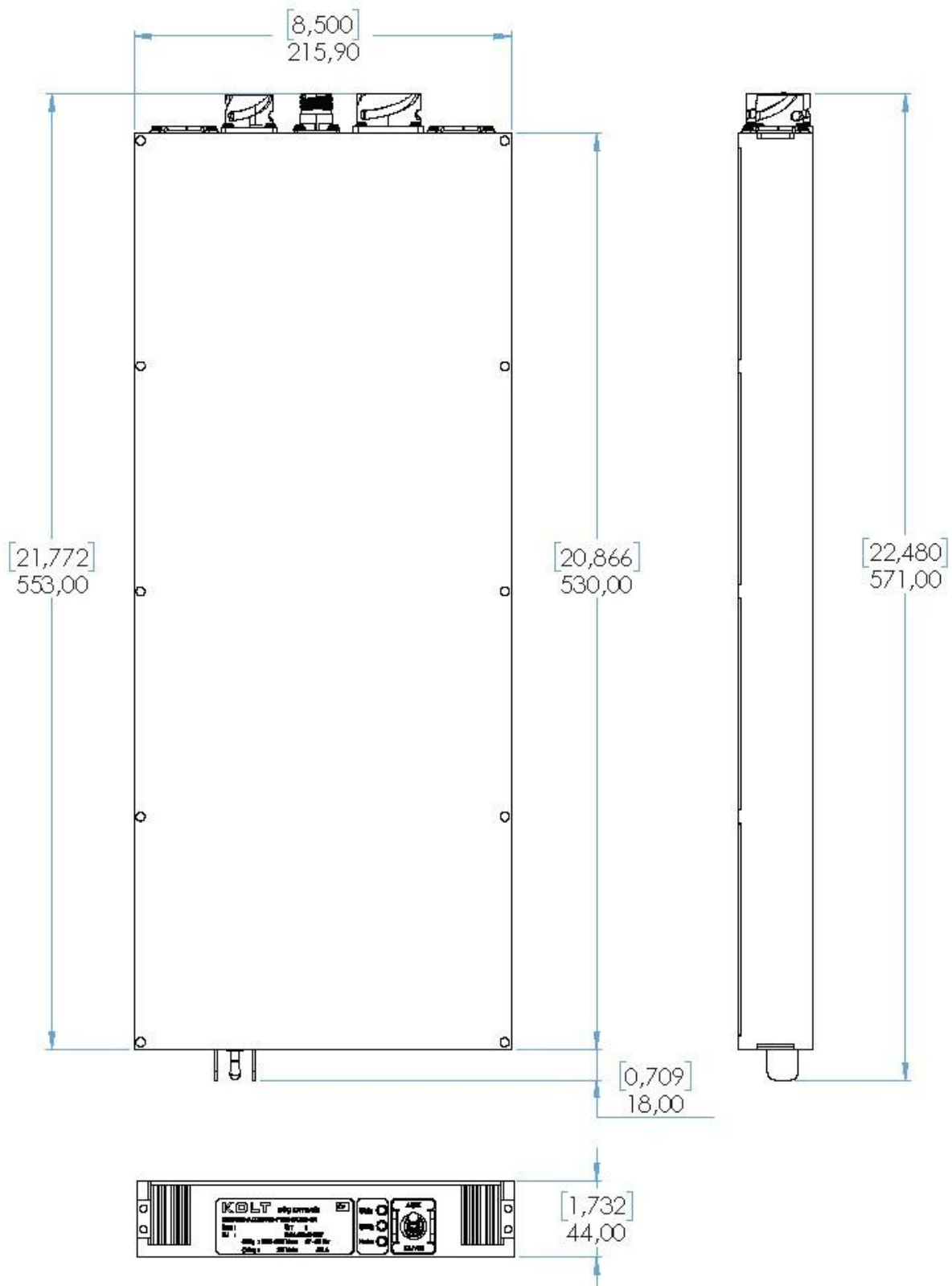
Figure 26. Mechanical Dimensions
