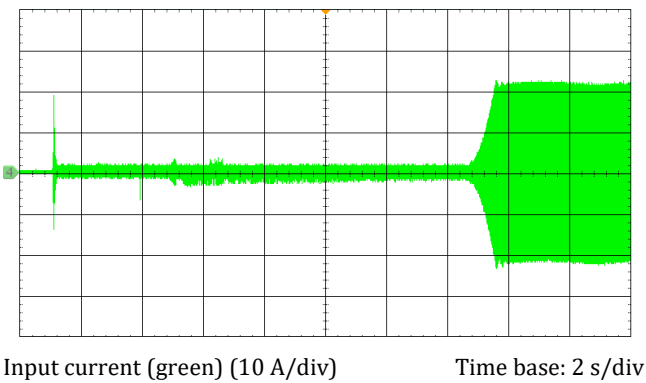
Figure 2. Input current for inrush and start-up stages at nominal input voltage
