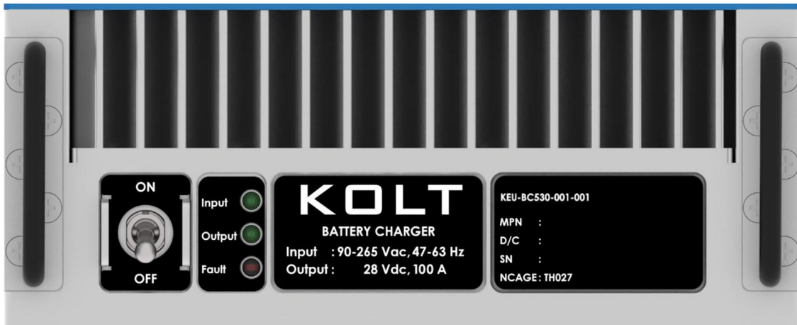
Figure 23. Front Panel
