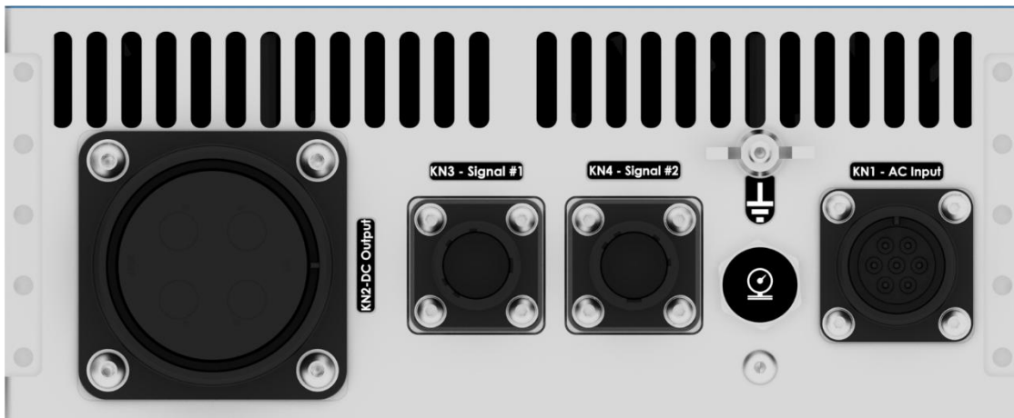
Figure 18. Connector Panel
