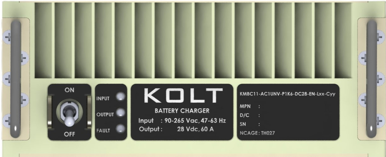
Figure 22. Front Panel
