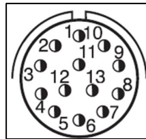
Figure 20. Signal Connector View
