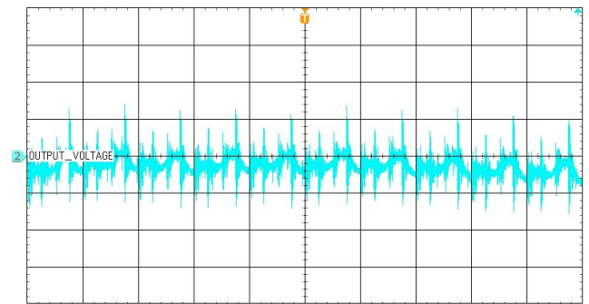
Output voltage (blue) (50 mV/div) Time base : 10 \mu s/div
