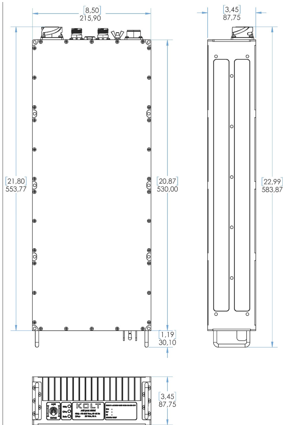
Figure 27. Mechanical Dimensions
