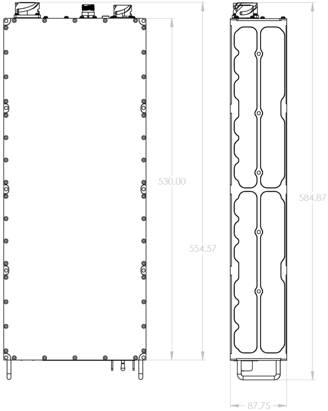
Figure 24. Mechanical Dimensions
