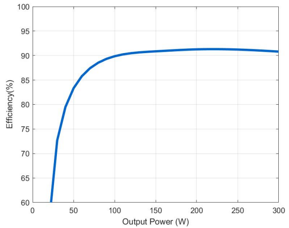
Figure 4. Efficiency versus output power at nominal input voltage (36 V)
