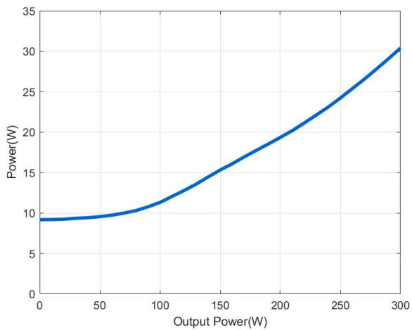
Figure 5. Power dissipation versus output power at nominal input voltage (36 V)
