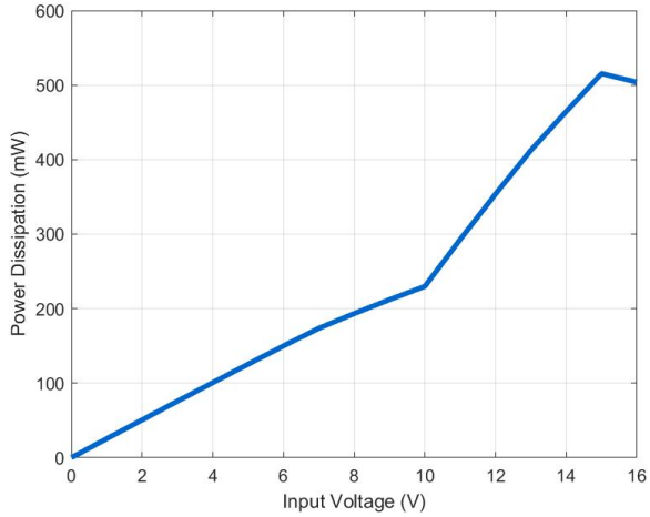
Figure 1. Disabled power dissipation versus input voltage
