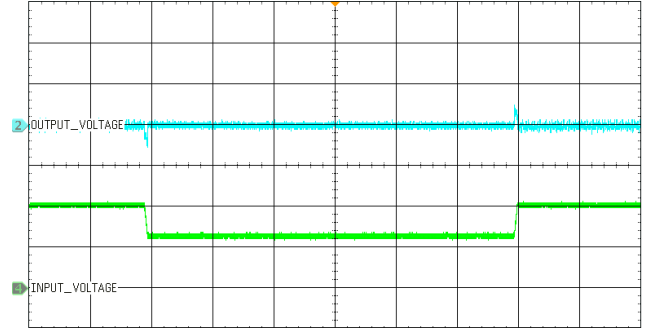
Output voltage (blue) (1 V/div) Time base : 200 ms/div Input voltage (green) (200 V/div)
