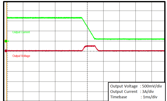
Figure 10. 100-10% Load Transient Response at Nom. V_{IN}
