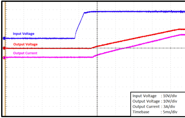
Figure 7. Input Voltage Start up Full Load
