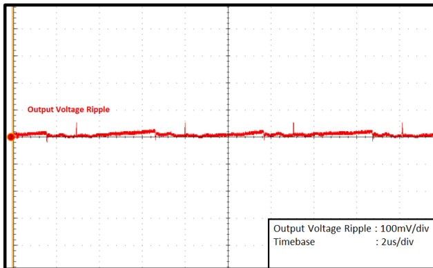
Figure 8.2. Output Ripple V_{in} = 28V Full Load
