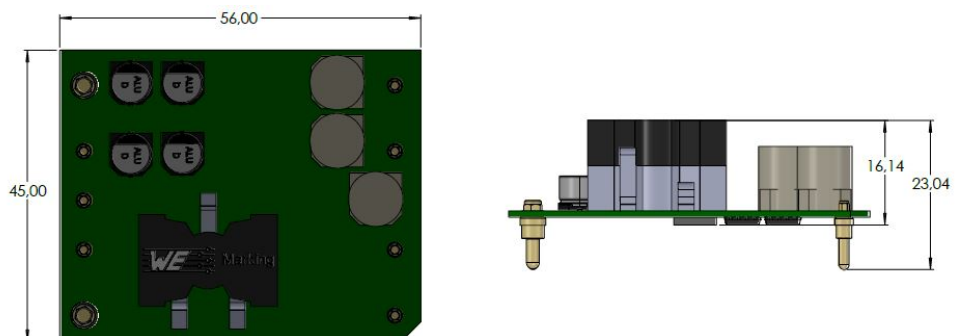
Outline Drawing(mm)
