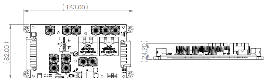
Outline Drawing(mm)
