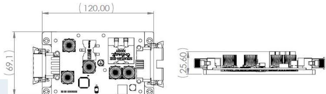
Outline Drawing(mm)
