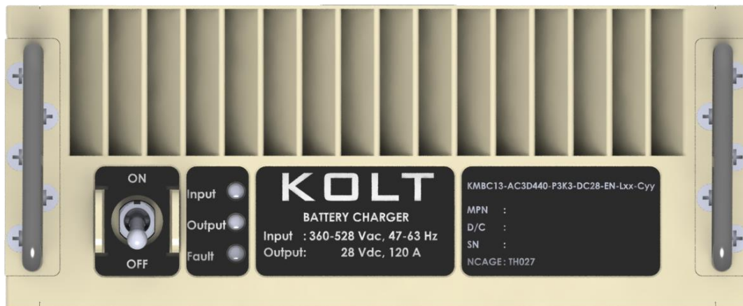
Figure 22. Front Panel
