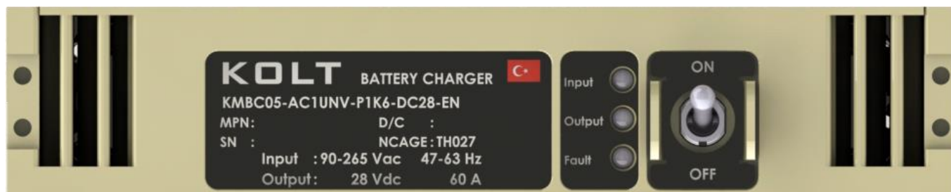
Figure 21. Front Panel
