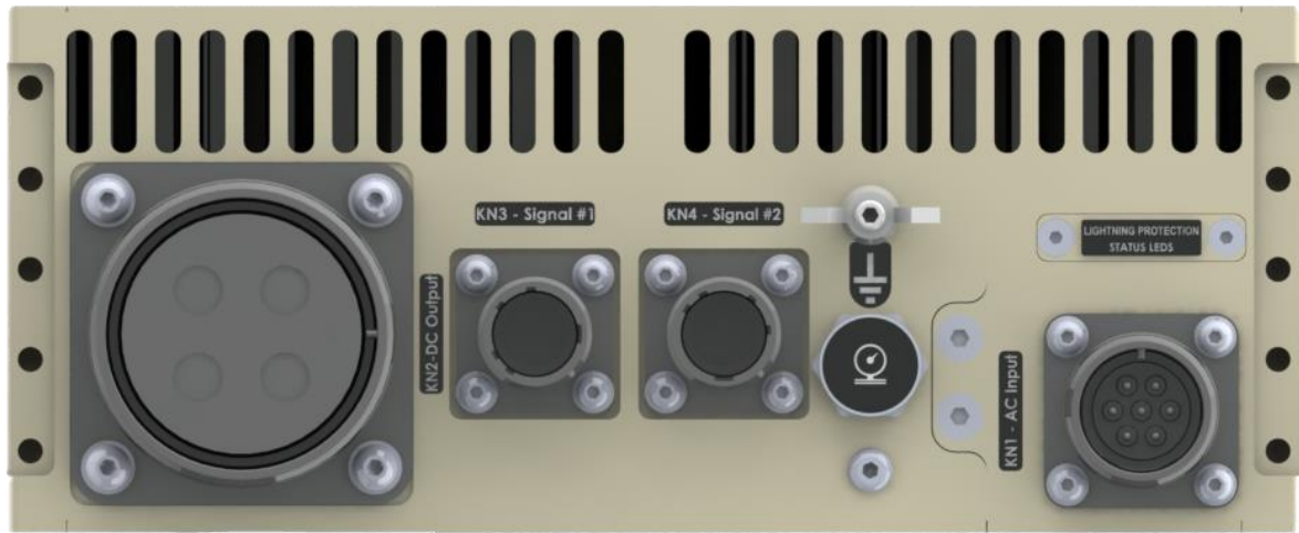
Figure 18. Connector Panel
