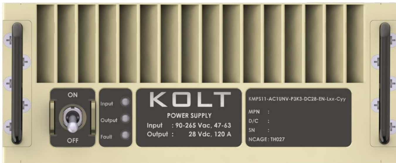
Figure 23. Front Panel
