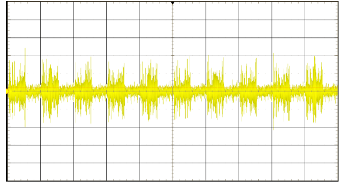
Leakage current (yellow) (10 mA/div) Time base: 20 ms/div
