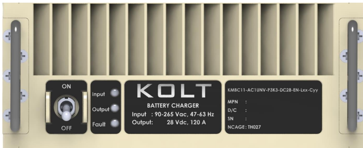
Figure 23. Front Panel
