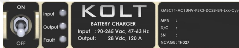
Figure 26. L02 Label Option Front View
