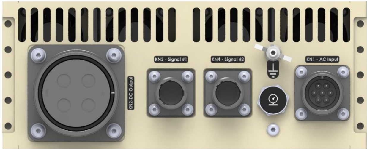
Figure 18. Connector Panel
