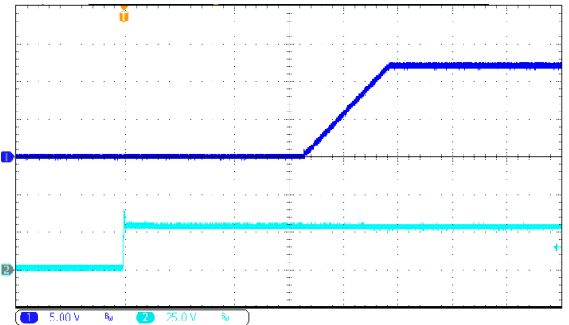
Output voltage (navy blue) (5 V/div) Time base: 20 ms/div Input voltage (cyan) (25 V/div)
