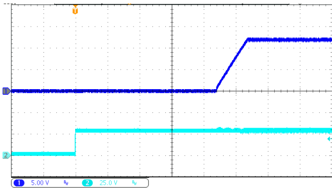
Output voltage (navy blue) (5 V/div) Time base: 20 ms/div ON/OFF pin voltage (cyan) (25 V/div)
