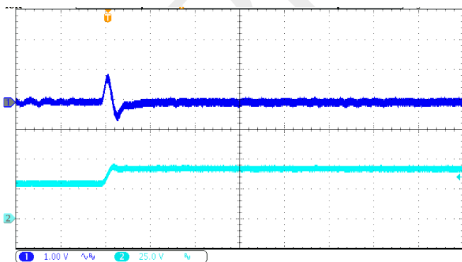
Output voltage (navy blue) (1V/div) Time base: 1 ms/div Input voltage (cyan) (25 V/div)
