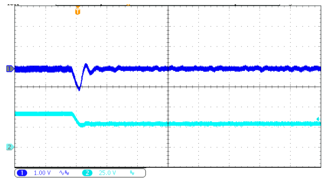
Output voltage (navy blue) (1V/div) Time base: 1 ms/div Input voltage (cyan) (25 V/div)
