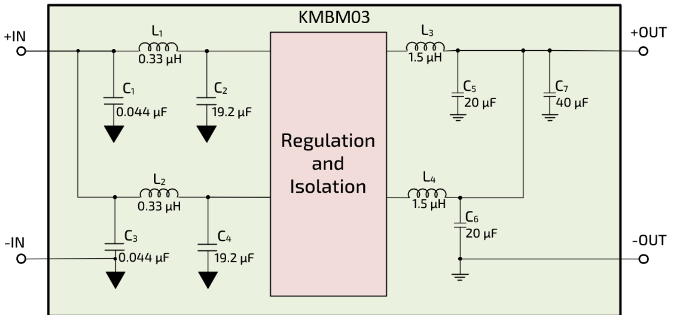
Figure V. Internal input and output filter diagram of KMBM03
